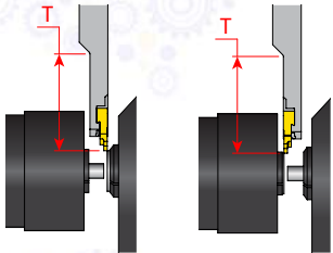
Figure 1 SR Tool - RH tool with RH insert Figure 2 SRS Tool - RH tool with LH insert
